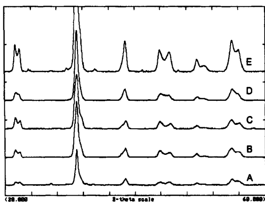
FIGURE 1 X-ray diffraction pattern of PZT powders, hydrothermally synthesized at different temperatures with a reaction time of 20 h A) 150 °C (20 nm) B) 175 °C (23 nm) C) 200 °C (21 nm) D) 225 °C (17 nm) E) 250 °C (20 nm)
