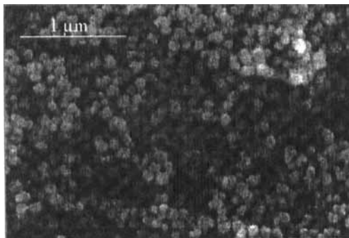
FIGURE 8 SEM picture of BaTiO 3 powder, density 5,5 g/cm 3 (91 % of th.), specific surface area 18 m 2 /g
